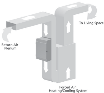
Return air direct plenum installation.
